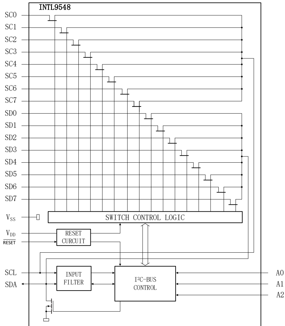
Figure 1 Functional Diagram
