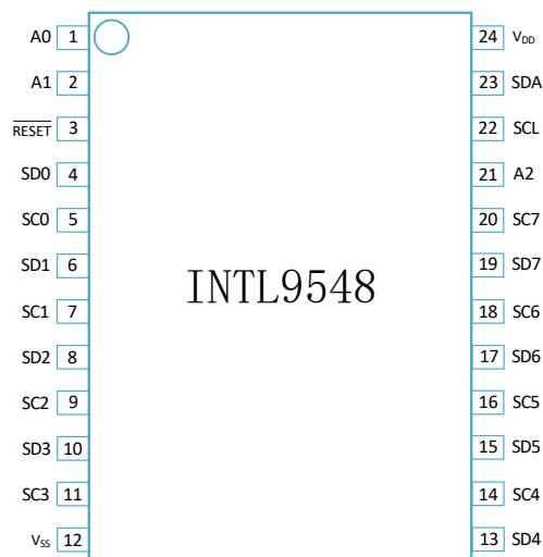
Figure 2 Pin Assignment Diagram
